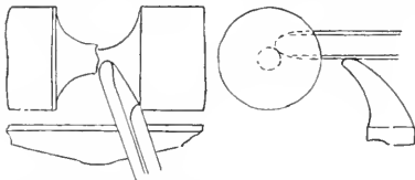
FIG. 314. FINAL POSITION OF GOUGE IN SHORT CONCAVE CUTS.
